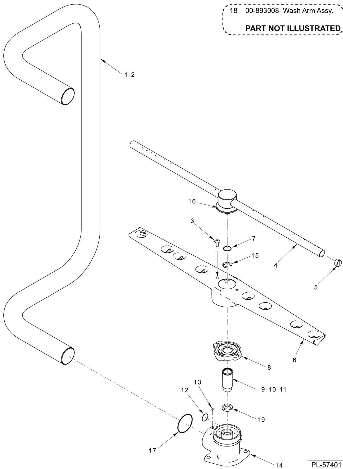
LOWER WASH ARM
