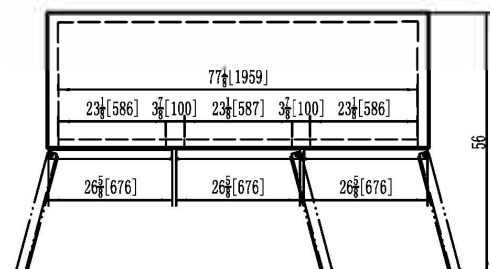
C-72FM-HC TOP VIEW
