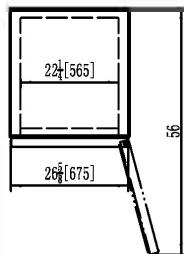
C-23FM-HC TOP VIEW
