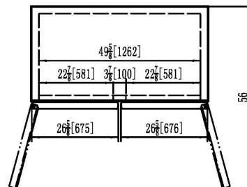
C-49FM-HCe TOP VIEW
