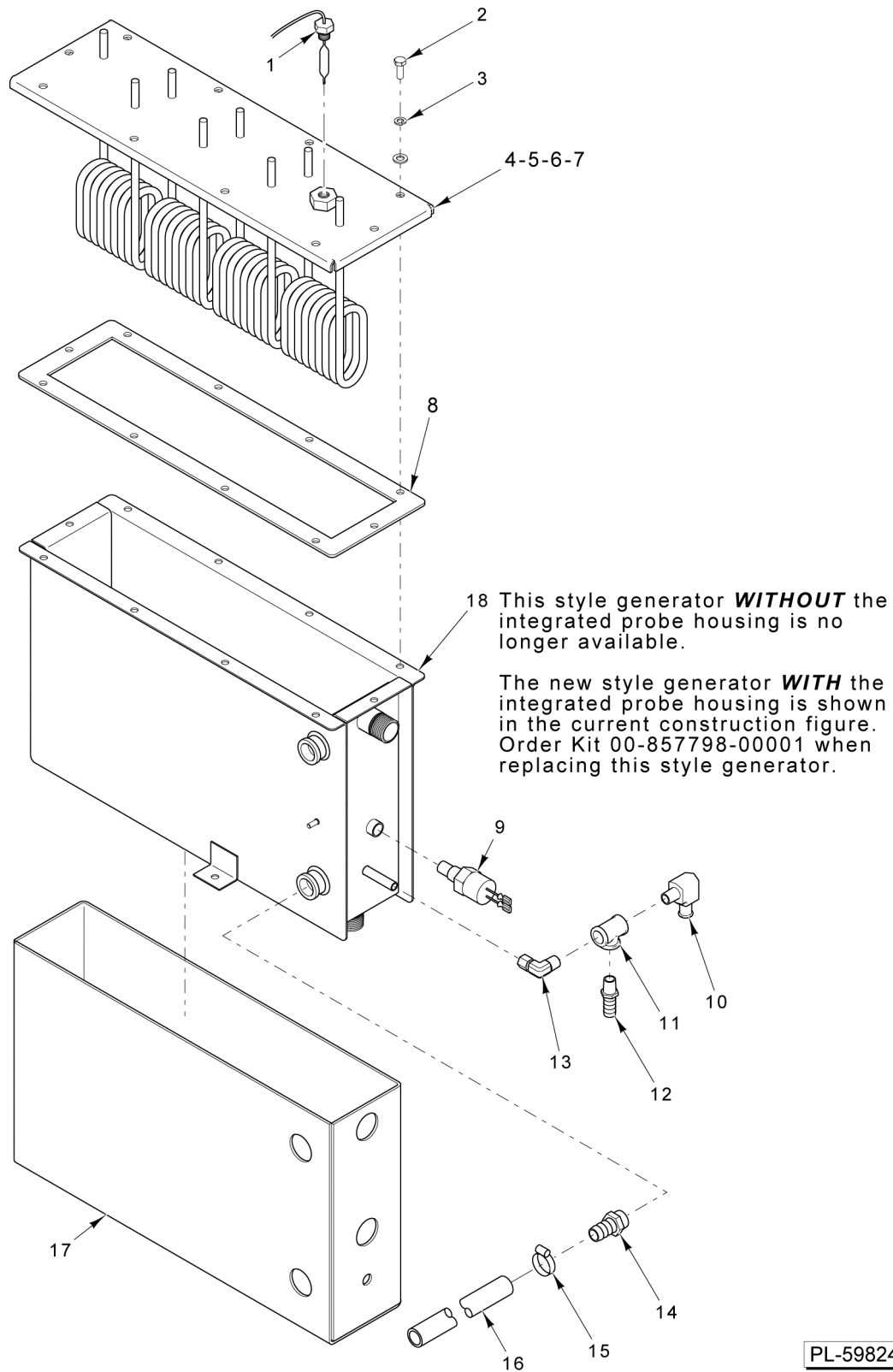
GENERATOR ASSEMBLY (PRIOR TO S/N 463003747)
