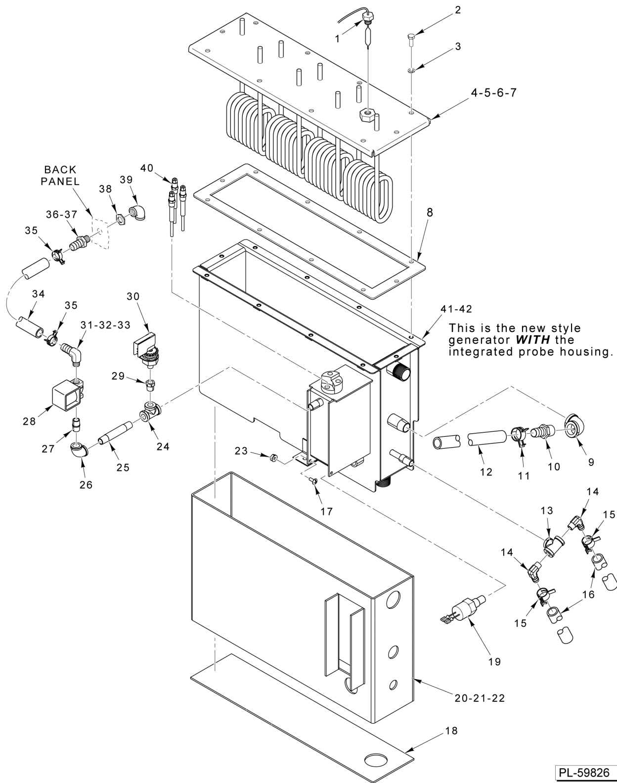
GENERATOR ASSEMBLY (AFTER S/N 463003747)
