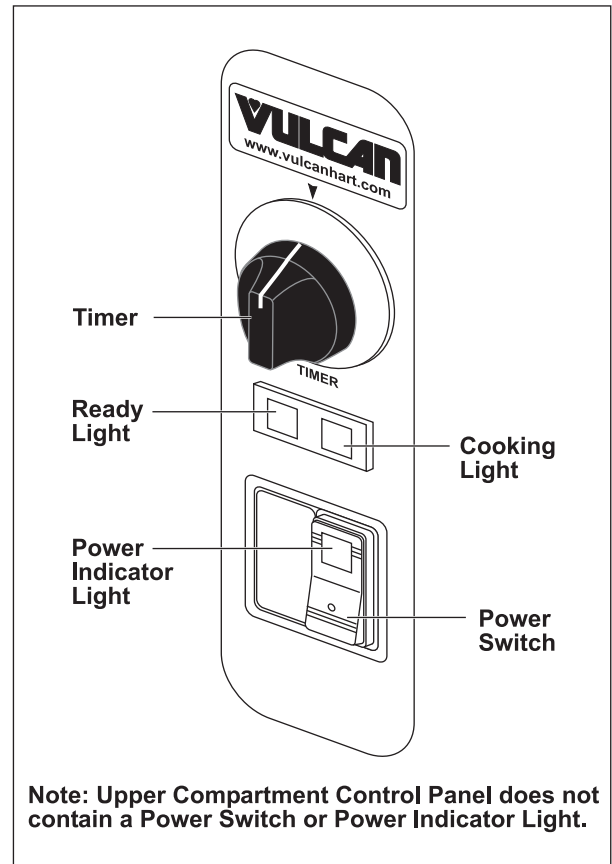
Figure 4. Cabinet Controls
