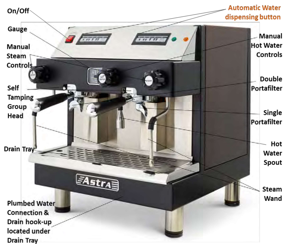
FIGURE 3: AUTOMATIC MEGA 1,2,3
