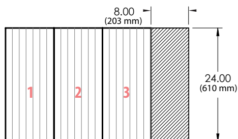
24 D x 42 L (610 x 1070 mm)
