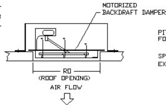
CURB DIMENSIONAL DATA
