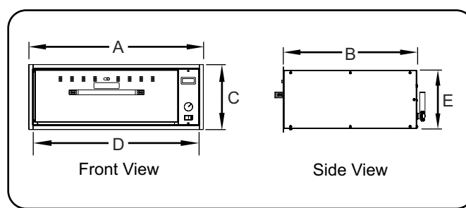
HDW-XB and HDW-XBN Dimensions
