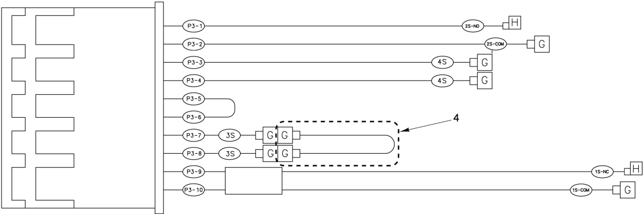
00-938462 Harness - Plug (J3) (HS6N-1R)
