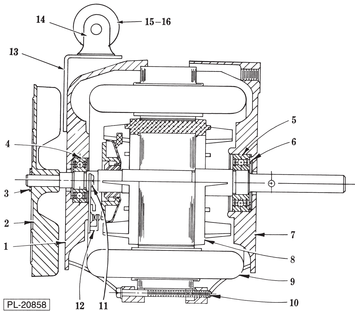
MOTOR UNIT
