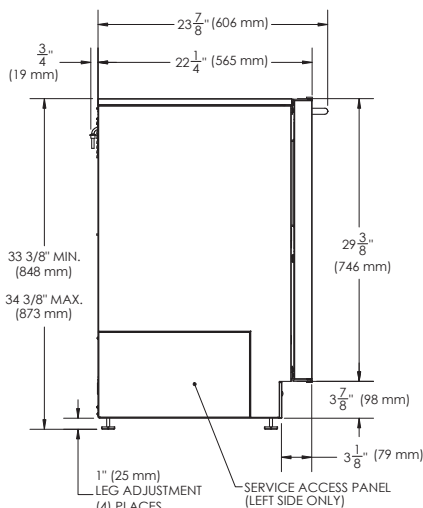
LEFT VIEW
