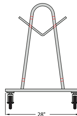
99360 All-Welded Cart
