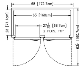
Plan - R/AIH232L
